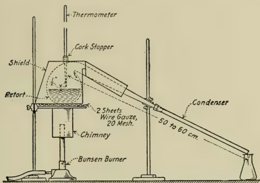
FIG. 187.—Retort Method of Distillation.
